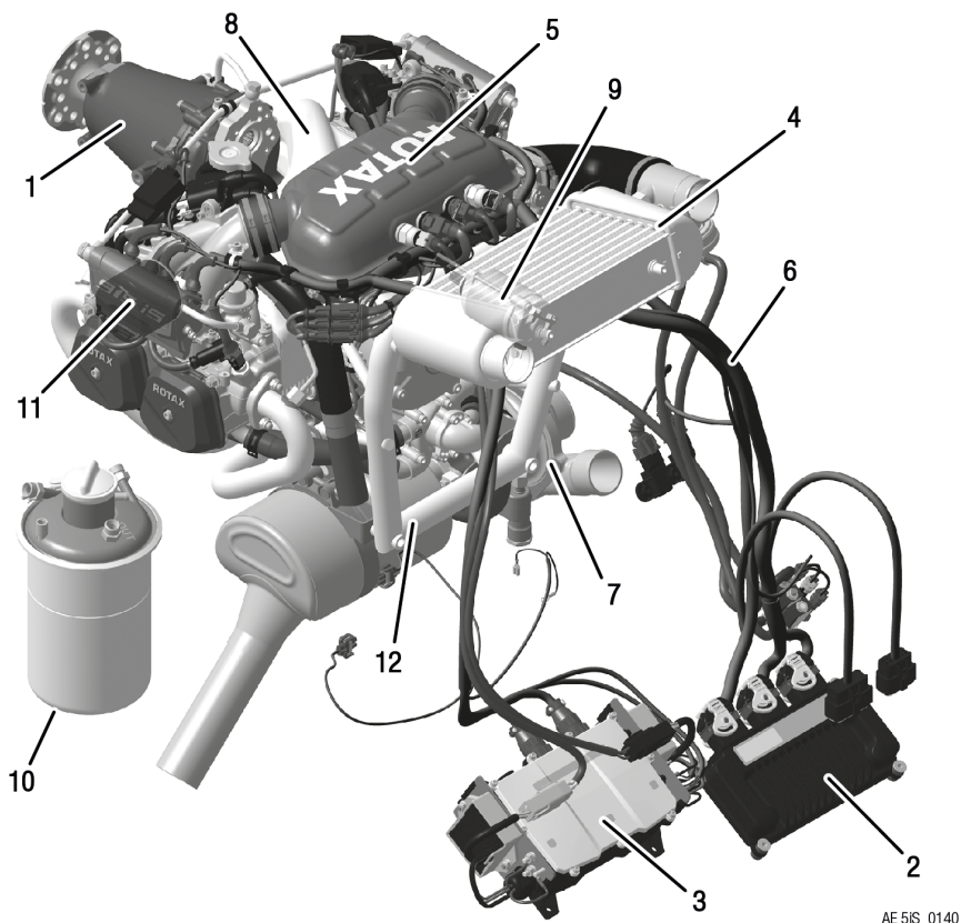
Figure 1: Engine components
