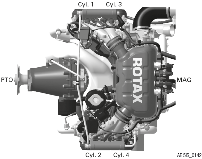
Figure 2: Cylinder arrangement
