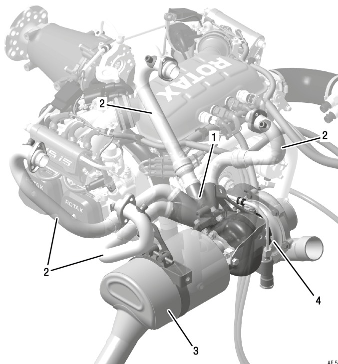
Figure 12: Turbocharger/Exhaust system
