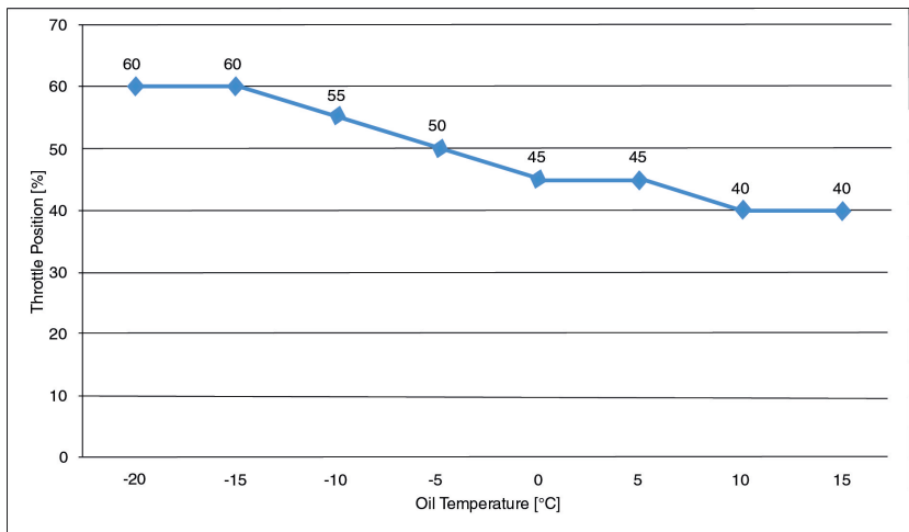
Figure 3: Throttle position
