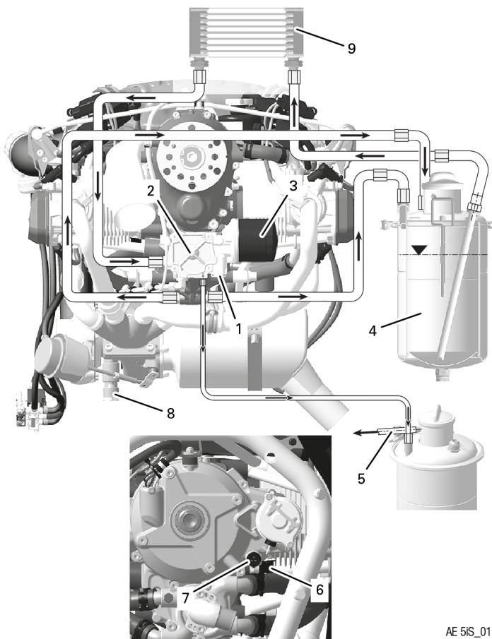
Figure 7: Lubrication system
